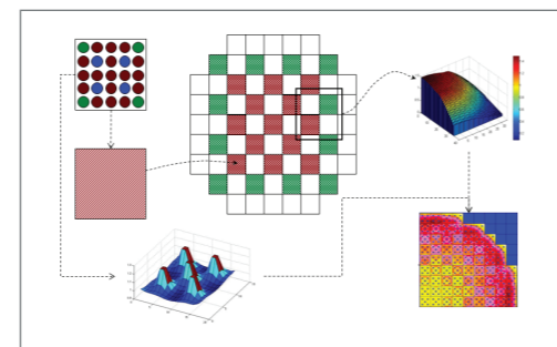
< Homogenization and Reconstruction of KARMA/ASTRA >
