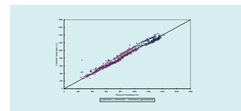
< Comparison of Calculated and Measured Fuel Centerline Temperatures >
