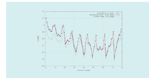
< THALES DNBR Calculation Accuracy >
